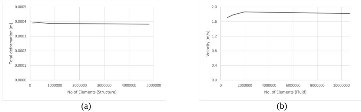
Fig. 5. Convergence study Solid domain (a); Fluid domain (b)
